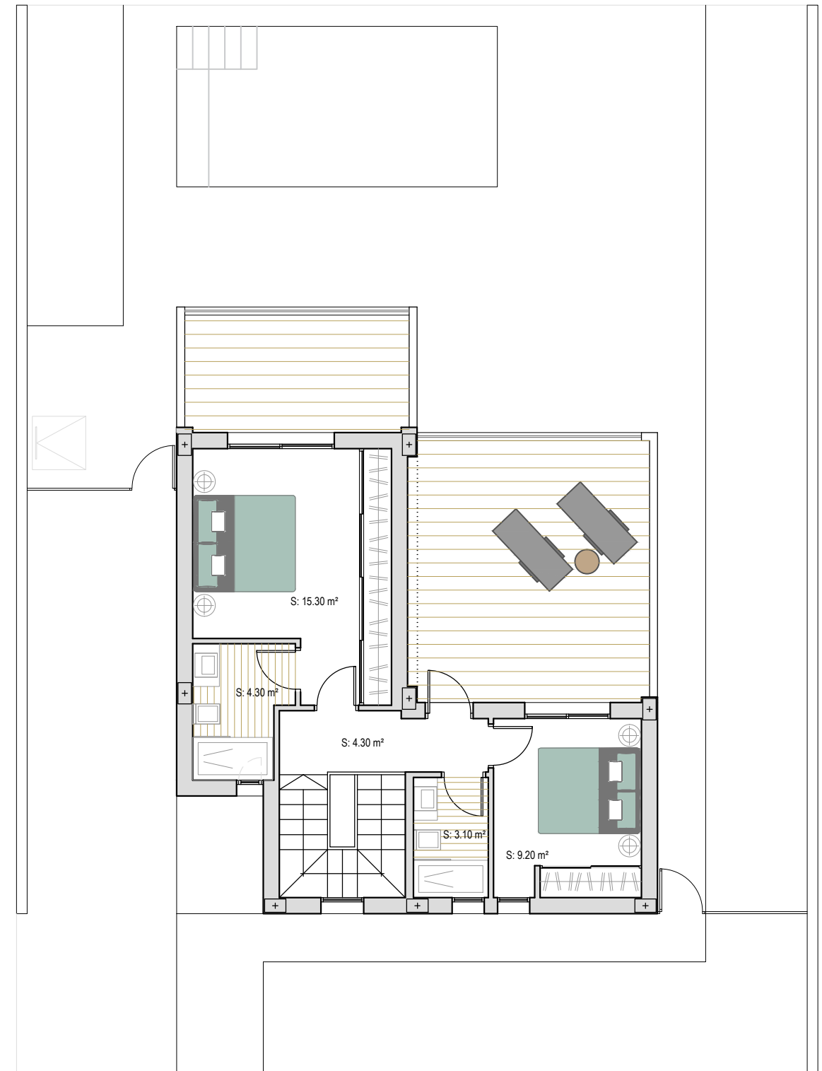
First floor
